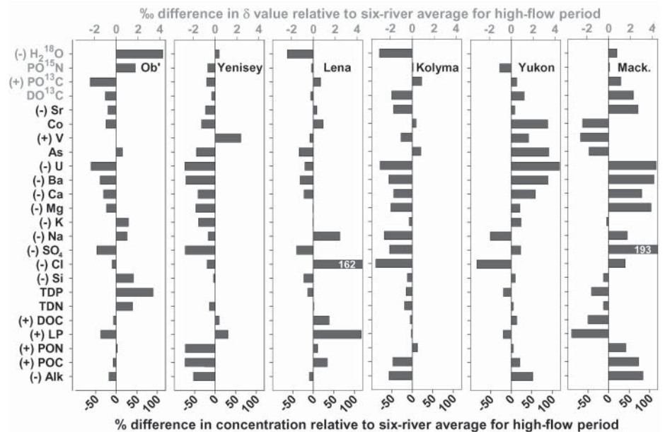
Fig. 1. Differences in chemistry among Pan-Arctic River Transport of Nutrients, Organic Matter, and Suspended Sediments (PARTNERS) rivers during high flow, late May through mid-June. Differences in isotope ratios are reported as \delta values (‰). All other differences are percentages. Plus signs in front of parameter labels indicate increases from low to high flow at all rivers, and minus signs indicate decreases from low to high flow. H_2^{18}O is the \delta^{18}O of water, PO^{15}N is the \delta^{15}N of particulate organic nitrogen (PON), PO^{13}C is the \delta^{13}C of particulate organic carbon (POC), DO^{13}C is the \delta^{13}C of dissolved organic carbon (DOC), TDP is total dissolved phosphorus, TDN is total dissolved nitrogen, Alk is total alkalinity, and LP is lignin phenols. Values for Alk, LP, strontium (Sr), cobalt (Co), vanadium (V), arsenic (As), uranium (U), barium (Ba), calcium (Ca), magnesium (Mg), potassium (K), sodium (Na), sulfate ( SO_4^{2-} ), chloride ( Cl^- ), and silicon (Si) are from filtered (0.45-micron) samples.
